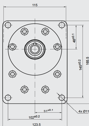
X SAE J 744 101-2 B \varnothing 101.6 mm
