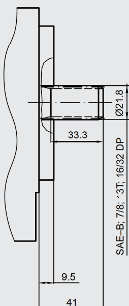
F Splined shaft SAE B - J 744 22-4 13T
