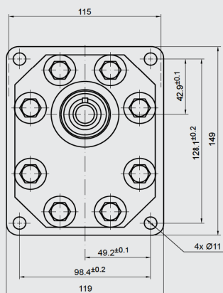
S Square flange centering \varnothing 50.8 mm
