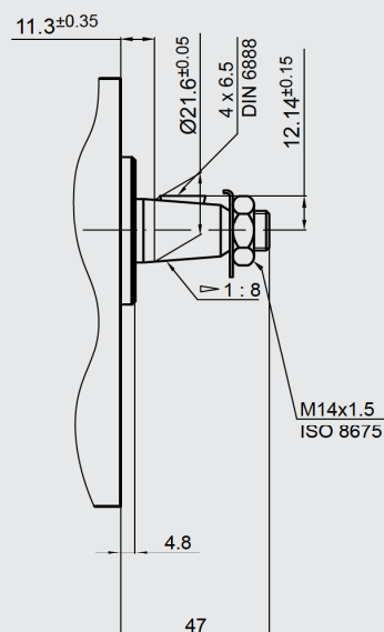
B Tapered keyed shaft 1:8
