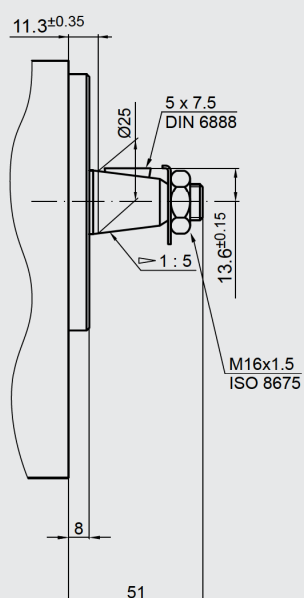
A Tapered keyed shaft 1:5
