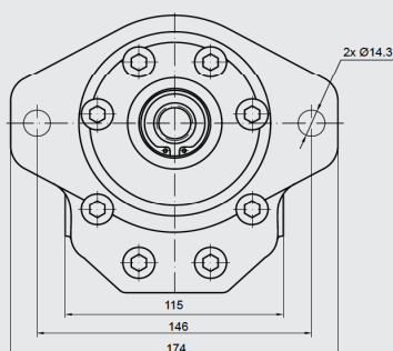
X SAE J 744 101-2 B \varnothing 101.6 mm
